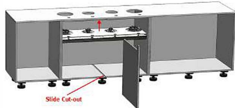
B1. Remove the center corpus from the cabinet and place the PITT Cooking unit inside the cabinet.
