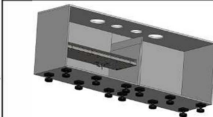
C2.1. Place the PITT Cooking unit inside the cabinet and manoeuvre it through the cut-out underneath the worktop. PAY ATTENTION! The cut-out has to be at least 250 mm high. (Measured from the bottom of the worktop)
